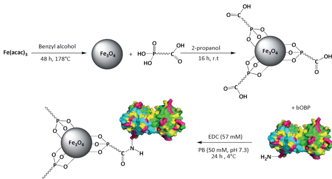
Fig. 2 Synthesis of bOBP-functionalized SPIONs.
