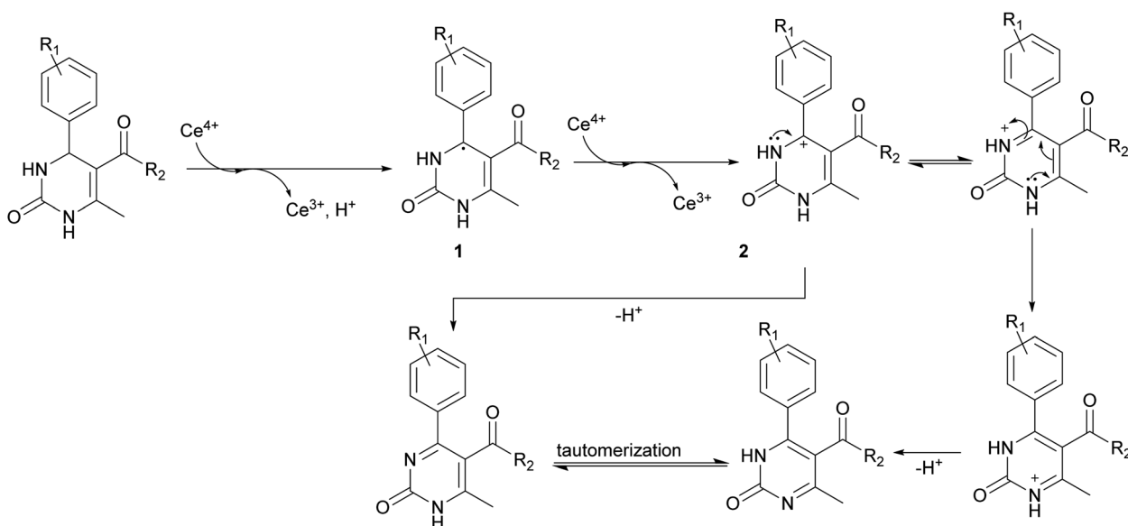
Scheme 6 Mechanism of regioselective oxidation of \text{H}_2\text{Py} in the presence of CAN.
