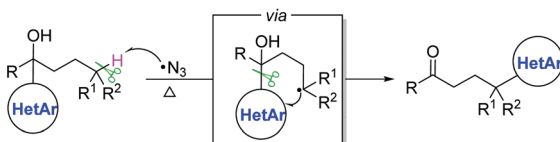
Scheme 1 Radical-mediated heteroarylation of unactivated C(sp 3 )-H bonds by means of functional group migration.
