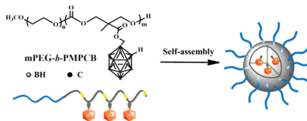
Scheme 1 Structure of the amphiphilic carborane-conjugated polycarbonate and self-assembly in water, adapted from ref. 20 with permission from the American Chemical Society, copyright 2016.
