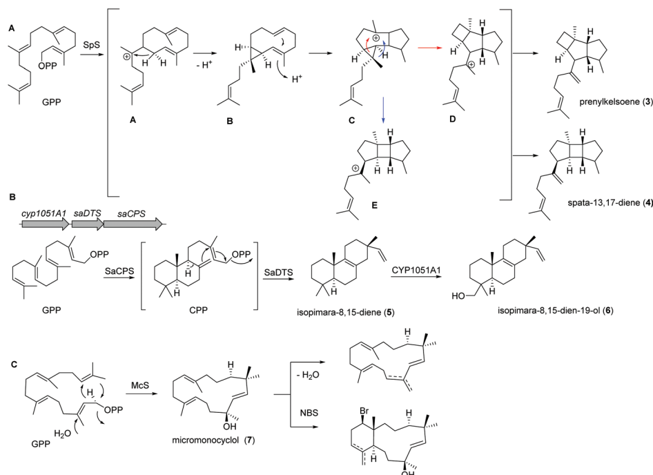
Fig. 3 (A) Biosynthesis of prenylkelsoene ( 3 ) and spata-13,17-diene ( 4 ) by spata-13,17-diene synthase (SpS) from Streptomyces xinghaiensis . (B) Biosynthetic pathway of isopimara-8,15-diene ( 5 ) and isopimara-8,15-dien-19-ol ( 6 ) in Salinispora arenicola ; (C) studies on the micromonocyclol synthase (McS) yielding micromonocyclol ( 7 ).
