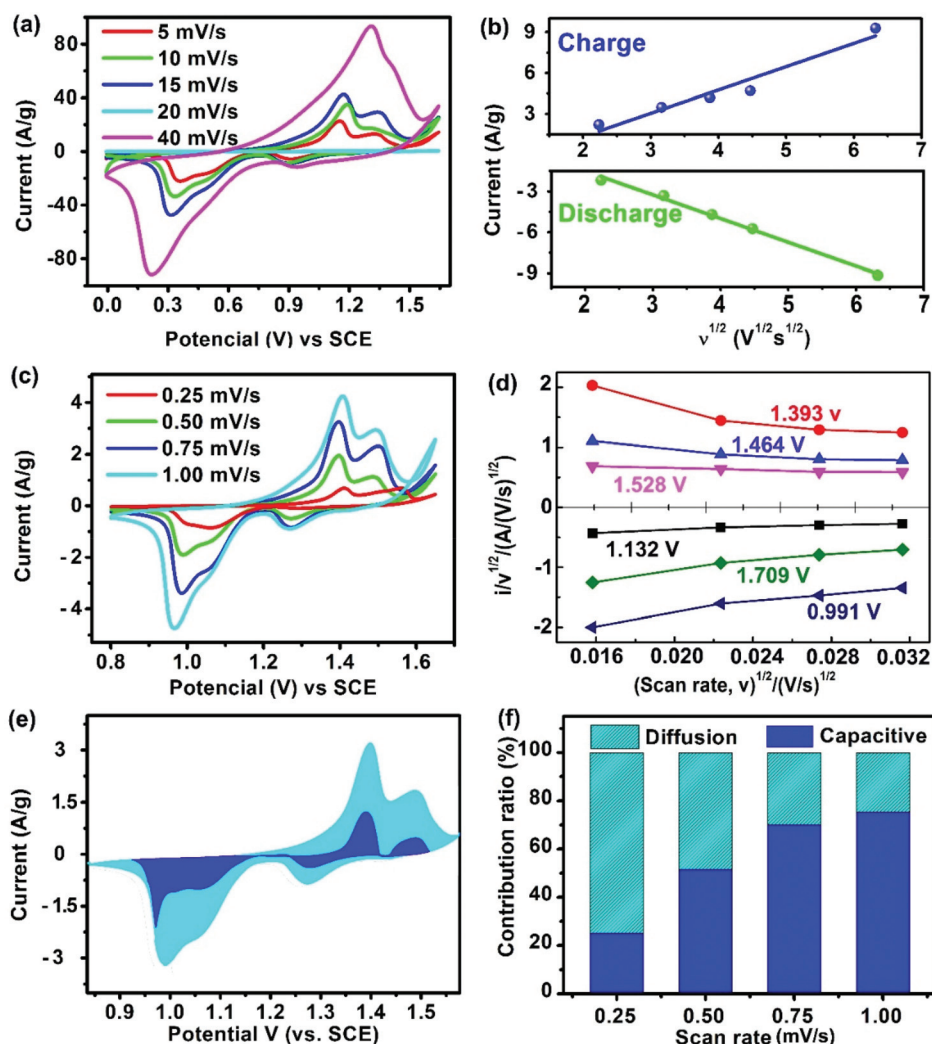
Fig. 4 (a) CV testing results of the NiAl-LDH/rGO/Co 3 O 4 @Fe 2 O 3 supercapacitor from 5 to 40 mV s -1 . (b) Relationship illustration of the peak currents and the \nu^{1/2} for the NiAl-LDH/rGO/Co 3 O 4 @Fe 2 O 3 supercapacitor. (c) CV testing results of the NiAl-LDH/rGO/Co 3 O 4 @Fe 2 O 3 supercapacitor from 0.25 to 1.00 mV s -1 . (d) Relationship illustration of \nu^{1/2} and i/\nu^{1/2} , the calculated k_1 and k_2 values were collected. (e) Charge storage contributions to the electrochemical capacitance at 0.75 mV s -1 . (f) Contribution ratios of the electrochemical capacitance of the NiAl-LDH/rGO/Co 3 O 4 @Fe 2 O 3 supercapacitor.
