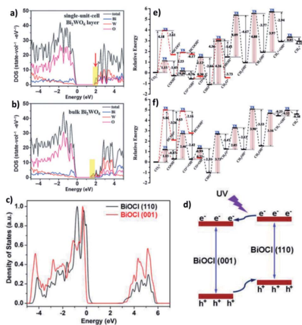
Fig. 25 (a) DFT calculations of Bi 2 WO 6 single-unit-cell layer slab and (b) bulk Bi 2 WO 6 slab. Reproduced with permission from ref. 213 Copyright 2015, Wiley-VCH. (c) PDOS diagrams from first-principles simulations for BiOCl (001) and (110) facets and (d) schematic showing the facet-dependent charge migration propensities in BiOCl. Reproduced with permission from ref. 87 Copyright 2015, Wiley-VCH. (e and f) Reaction pathways for CO 2 reduction to CH 4 on BOC-OV and BOC, respectively, where "*" represents adsorption on the substrate. The red route is the alternative pathway. Reproduced with permission from ref. 211 Copyright 2017, The Royal Society of Chemistry.
