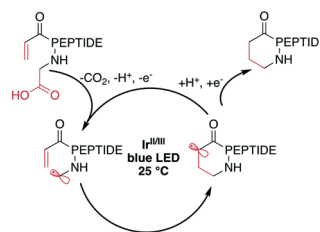
Scheme 25 Simplified reaction mechanism for the Ir-photocatalyzed macrocyclization of N -acroyl peptides.
