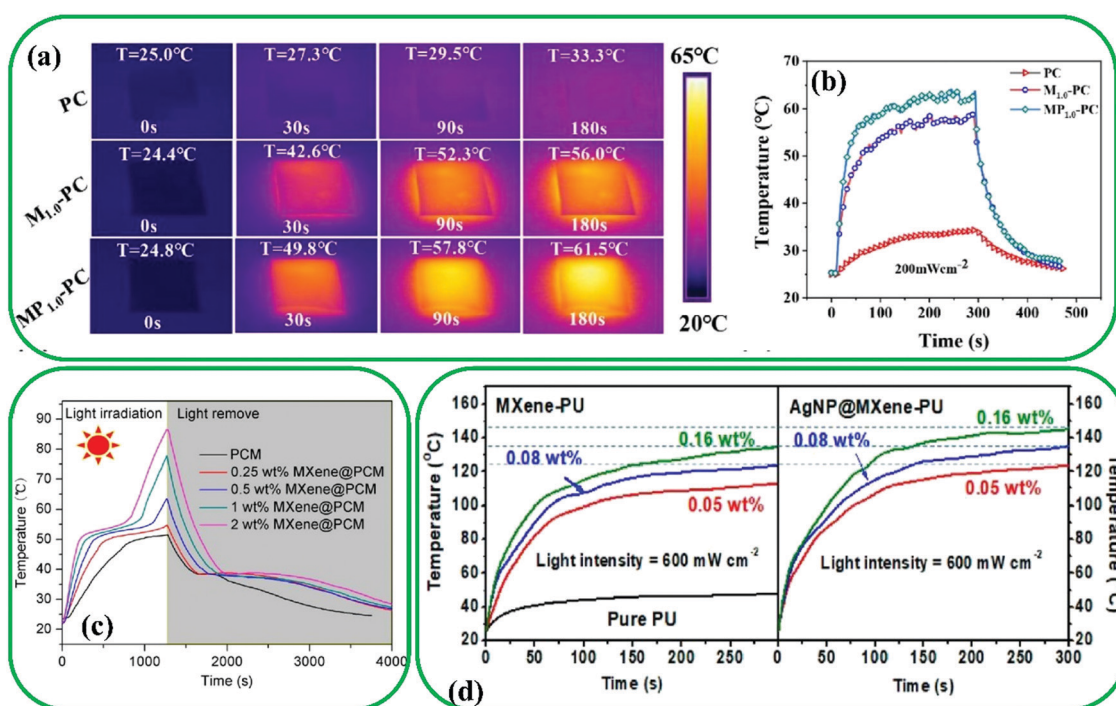
Fig. 20 (a) IR thermal images and (b) surface temperature evolution curves of different \text{MXene@PPy} -based films under 200 \text{ mW cm}^{-2} . Reproduced with permission. 239 Copyright 2021, American Chemical Society. (c) Temperature evolution curves of pristine PCM and \text{MXene@PCM} at different concentrations of \text{Ti}_3\text{C}_2 . Reproduced with permission. 240 Copyright 2020, American Chemical Society. (d) Temperature changes as a function of time for \text{MXene-PU} (left) and \text{AgNP@MXene-PU} (right) under 600 \text{ mW cm}^{-2} . Reproduced with permission. 241 Copyright 2019, American Chemical Society.
