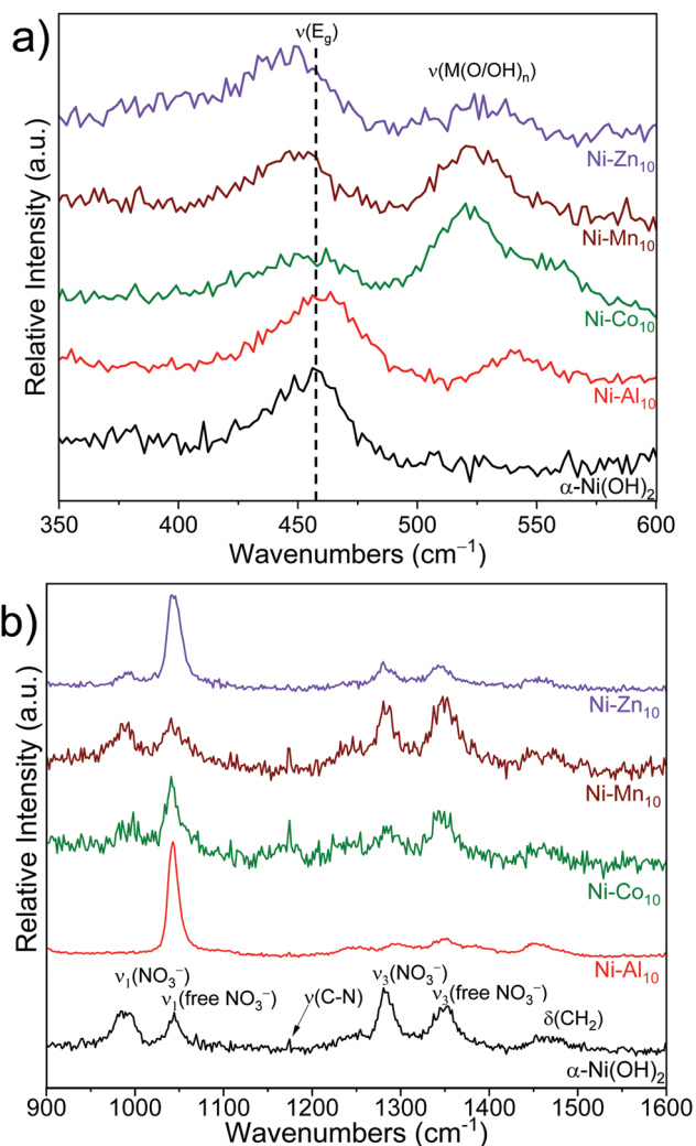
Fig. 3 Raman spectra of unsubstituted \alpha -Ni(OH) _2 , aluminum-substituted (Ni-Al _{10} ), cobalt-substituted (Ni-Co _{10} ), manganese-substituted (Ni-Mn _{10} ), and zinc-substituted (Ni-Zn _{10} ): (a) 350 \text{cm}^{-1} to 600 \text{cm}^{-1} spectral region and assignments of lattice modes; (b) 900 \text{cm}^{-1} to 1600 \text{cm}^{-1} spectral region and assignments of modes from compounds incorporated into the structure.
