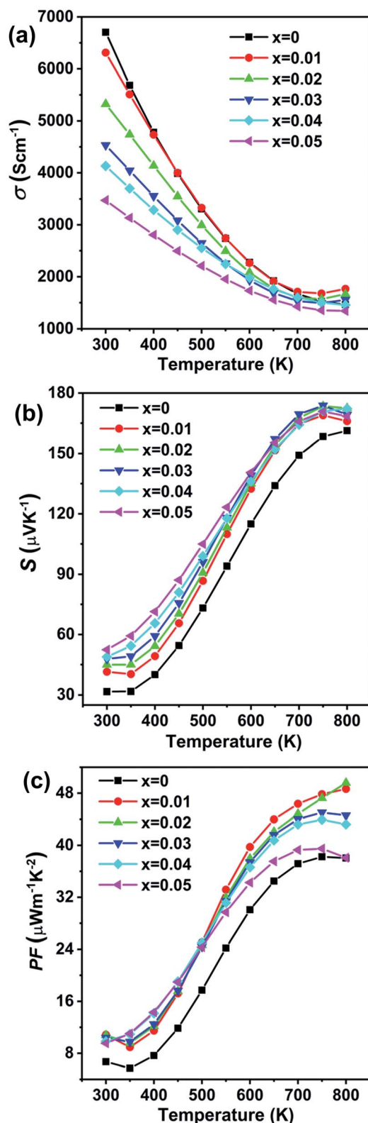
Fig. 4 Electronic transport properties as a function of temperature for Ge 1-x Cd x Te ( x = 0-0.05 ) samples: (a) electrical conductivity, (b) Seebeck coefficient, (c) power factor.
