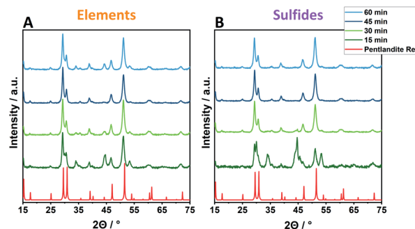
Fig. 1 Exemplified powder X-ray diffractograms of Pn-materials synthesized at different time scales (15–60 min) using 8 \times 10 mm \text{ZrO}_2 balls and starting from an elemental reaction mixture (A, \text{E}_8 -Y) or the respective metal sulfides (B, \text{S}_8 -Y).
