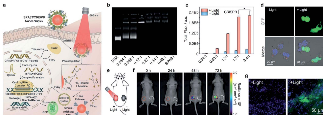
Fig. 10 (a) Schematic illustration of SPA33-mediated delivery and photoregulation of CRISPR/Cas9 gene editing. (b) Agarose gel electrophoresis of DNA, SPA33 and DNA/SPA33 complexes at different N/P ratios. (c) Total fluorescence of GFP for SPA33/CRISPR complexes at different N/P ratios with or without 680 nm laser irradiation. (d) Confocal fluorescence images of SPA33/CRISPR-transfected cells with or without 680 nm laser irradiation. (e) Schematic illustration of laser irradiation for living mice. (f) Fluorescence images of mice at different post-irradiation times with (red circles) or without (white circles) 680 nm laser irradiation. The red/white circles indicate the regions with subcutaneously implanted Matrigel mixed HeLa cell pellets transfected with SPA33/CRISPR with/without laser irradiation. (g) Confocal fluorescence images of Matrigel mixed cell pellet slices from mice with or without laser irradiation at t = 72 h post-treatment. The blue, green and red fluorescence indicate nuclei, GFP and SPA33, respectively. Error bars represent the standard deviations of three different measurements. *No statistically significant difference. Adapted from ref. 138. Copyright© 2019 Wiley-VCH Verlag GmbH & Co. KGaA, Weinheim.
