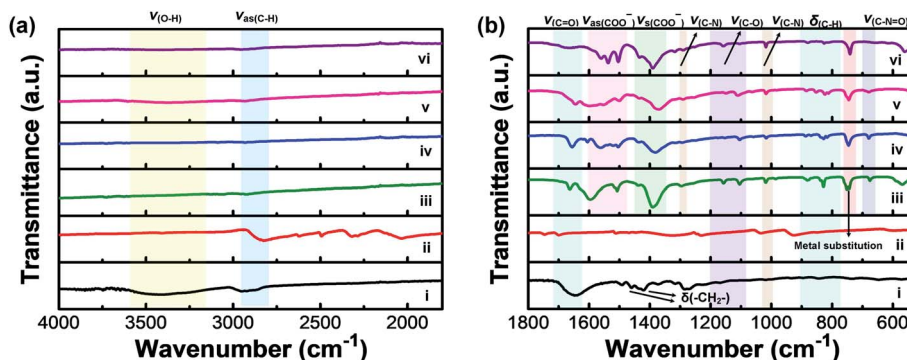
Fig. 2 FTIR spectra of (i) pure PVP, (ii) H 2 BDC ligand and the as-prepared M-BDC products: (iii) Cu-BDC, (iv) Mn-BDC, (v) Ni-BDC, and (vi) Zr-BDC in the wavenumber regions of (a) 4000–1800 cm -1 and (b) 1800–525 cm -1 .
