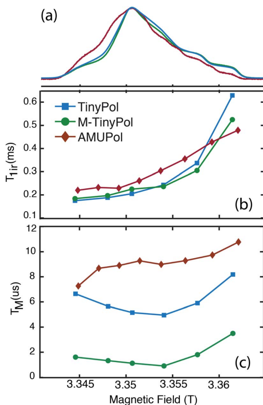
Fig. 5 (Top) W-band ( \sim 94 GHz) echo-detected EPR spectra of 100 \mu M TinyPol, M-TinyPol and AMUPol solutions in d_8 -glycerol/ D_2O / H_2O 60/30/10 (v/v/v) recorded at 100 K. (Middle) Electron spin lattice relaxation time ( T_{1e} ) and (bottom) electron phase memory time ( T_m ) measured at various position of the magnetic field. See ESI for Experimental details.†
