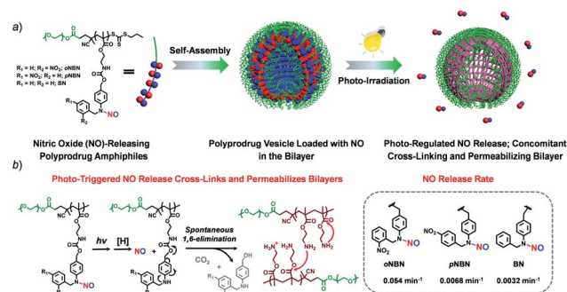
Scheme 1 (a) Schematic illustration of the formation of vesicles assembled from NO-releasing amphiphiles. The resulting vesicles encompass photoresponsive N -nitrosoamine moieties within the bilayer membranes shielded by hydrophilic PEO coronas. (b) Under light irradiation, the cleavage of N–NO bonds induces the 1,6-elimination reaction with the release of primary amine groups that further undergo inter/intrachain amidation reactions, concomitantly cross-linking and permeabilizing the bilayers.
