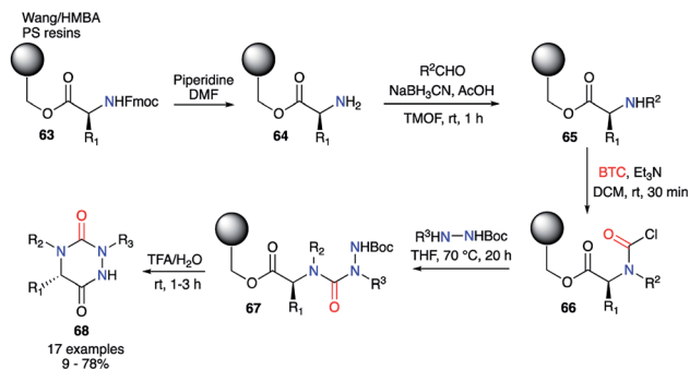
Scheme 22 Aza-DKP synthesis on Wang or HMBA resin (PS = polystyrene).
