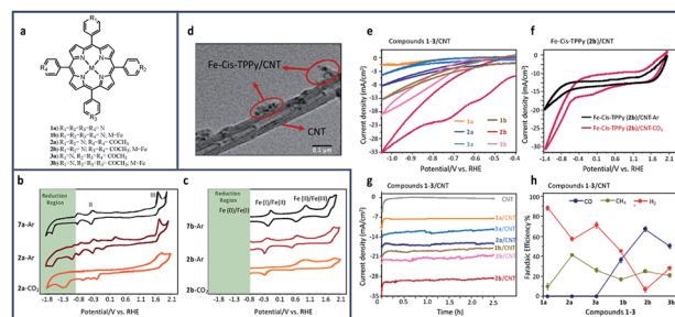
Fig. 11 (a) Molecular structure of pyridine-porphyrin complexes (b) CV comparison of 0.01 mM of TPP (7a)/GCE under argon, and cis -TPPy (2a)/GCE under argon and \text{CO}_2 ; (c) Fe-TPPy (7b)/GCE under argon, and Fe- cis -TPPy (2b)/GCE under argon and \text{CO}_2 in 0.1 M \text{NBu}_4\text{PF}_6/\text{DMF} solution. Conditions: scan rate: 100 \text{ mV s}^{-1} ; working electrode: glassy carbon; reference electrode: Ag/AgCl; counter electrode: platinum; (d) Transmission electron microscopy (TEM) image of the porphyrin 2b/CNT with scale bar of 0.1 \mu\text{m} . CV comparison of (e) all compounds 1-3/CNT under \text{CO}_2 ; (f) compound 2b/CNT in the presence and absence of \text{CO}_2 ; (g) chronoamperometry comparison of 1-3/CNT at -0.6 \text{ V vs. RHE} ; (h) FE comparison of all 1-3/CNT compounds at -0.6 \text{ V vs. RHE} in 0.1 M aqueous \text{NaHCO}_3 . 17 Copyright (2020) American Chemical Society.
