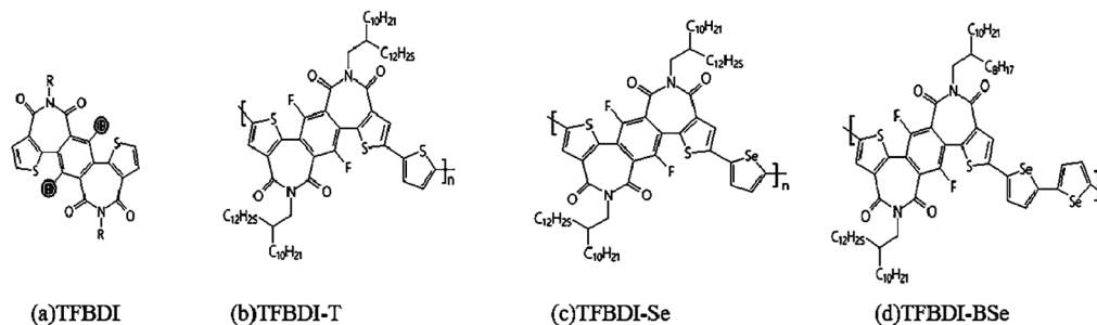
Fig. 7 Some monomers of fluorinated dithienylbenzodiazepines (a–d).
