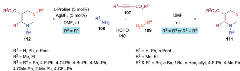
Scheme 24 One-pot multi-component divergent synthesis of polysubstituted tetrahydropyrimidines.
