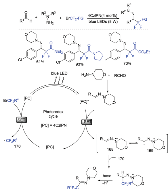
Scheme 114 The three-component difluoroalkylation reaction between aldehydes, hydrazines and halodifluoromethylated reagents.
