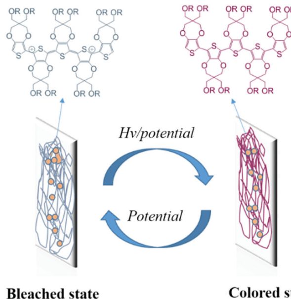
Fig. 75 Trifunctional CdSe quantum dots-polymer composite film with electrochromic, electrofluorescent, and light-induced coloration effects. Adapted from ref. 543 with permission. Copyright (2018) from Elsevier Ltd.
