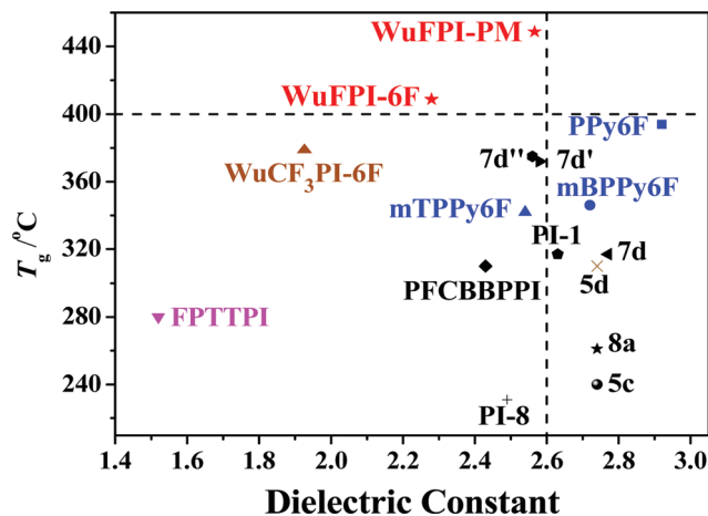
Fig. 34 Relationship between k and T_g of the polyimides developed by Zhang's group and the reported intrinsic low- k polyimides. Reprinted from ref. 260 with permission. Copyright (2019) Springer.
