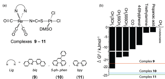
Fig. 6 (a) Structures of complexes 9–11; (b) binding strengths ( \Delta G^\circ ) of the [Pt^{II}(DMSO)Cl_2] -analyte adducts. The three horizontal lines represent the \Delta G^\circ values of complexes 9–11.
