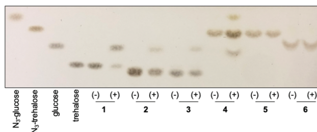
Fig. 2 Activity of M. smegmatis trehalase with trehalose 1 and trehalose derivatives (2–6). Compounds were incubated in the absence (–) or presence (+) of the M. smegmatis trehalase enzyme for 19 h. Mannotrehalose (2), galactotrehalose (3), azido-trehalose (4), azido-mannotrehalose (5) and azido-galactotrehalose (6).
