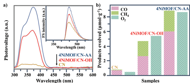
Fig. 4 SS-SPS responses and FS spectra (inset) related to the amount of produced \cdot\text{OH} (a) and the photocatalytic activities for \text{CO}_2 conversion under visible-light irradiation for 4 hours (b) of CN, 4NiMOF/CN-OH and 4NiMOF/CN-AA.
