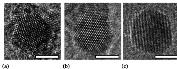
Fig. 9 Nanoparticle HRTEM micrographs of sample (a) A, (b) B and (c) C (scale bar = 3 nm).
