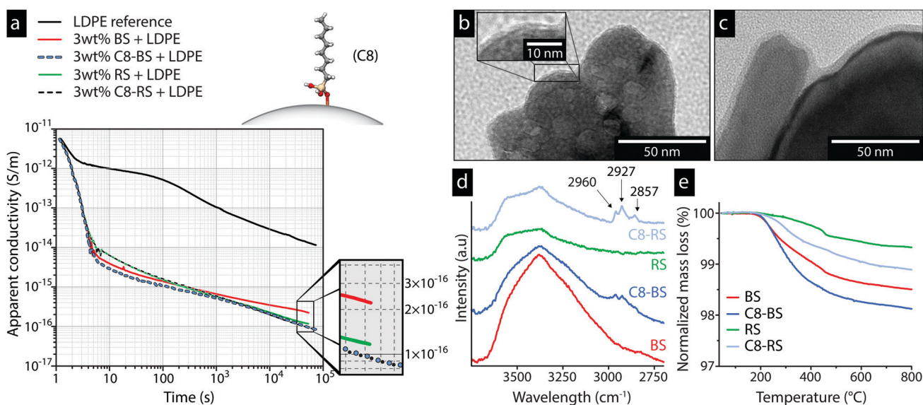
Fig. 6 (a) Apparent conductivity of LDPE composites containing 3 wt% C8 modified ball- or rod-shaped ZnO particles measured at 60 ^{\circ}\text{C} and 30 \text{kV mm}^{-1} . The inset in (a) illustrates the molecular structure of the C8 silsesquioxane bonded to the surface. The electron micrographs show (b) ball-shaped particles with 2 nm coatings and (c) rod-shaped particles with 5 nm coatings. Characterization of the C8 functional silsesquioxane encapsulated particles by infrared spectroscopy is shown in (d) and by thermogravimetry in (e). The inset in (b) shows a magnification of the C8 coating on ball-shaped particles. The presence of alkyl groups from the hydrocarbon tail of the silsesquioxane were confirmed by the peaks at 2800–3000 \text{cm}^{-1} assigned to the stretching vibrations of C–H bonds. 15,37 Table S1 (ESI † ) lists the measured conductivities, and additional micrographs of the unmodified particles are shown in Fig. S5 (ESI † ).
