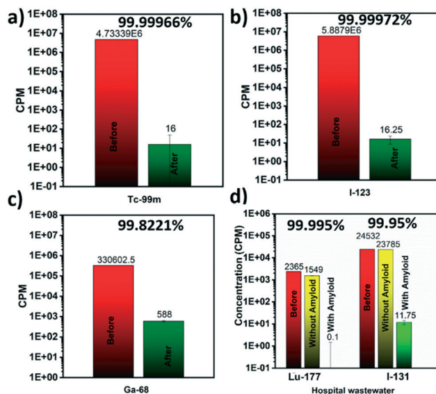
Fig. 2 Removal efficiencies for the different radioactive substances. Aqueous solutions filtered by amyloid–carbon hybrid membranes using syringe aided setup for: (a) Tc-99m pertechnetate, (b) I-123, (c) Ga-68, and (d) hospital wastewater having the mixture of Lu-177 and I-131.
