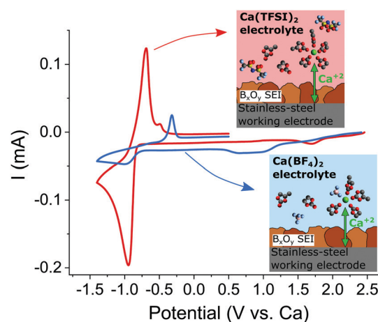
Fig. 6 Cyclic voltammograms ( 0.1\text{ mV s}^{-1} ) of pre-passivated stainless-steel electrodes (covered with borate films) using either Ca(TFSI)_2 (red curve) or Ca(BF_4)_2 (blue curve) electrolytes. Insets show the proposed cation solvation structures in each electrolyte, which are expected to be responsible for the difference in electrochemical behaviour between the two electrolytes.
