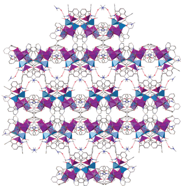
Fig. 5 View of the ab plane in the extended structure of 6 showing hydrogen bonding interactions (dashed red lines) between ligated and co-crystallised dmf and the overall bi-layer type array. Colour code C – grey, O – red, N – royal blue, Mn^{II} – pale blue polyhedra, Mn^{III} – purple polyhedra. Hydrogen atoms not involved in H-bonding, tBu groups, ligated solvent molecules and co-crystallised solvent/anions omitted for clarity.
