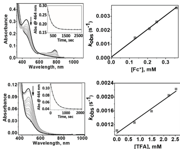
Fig. 7 Top: Changes in the absorption band associated with the reaction of 1 (0.015 mM) with TFA (3 mM) and \text{Fc}^* (0.15 mM) at -50^\circ\text{C} ; Inset: The pseudo-first order decay of the absorption band at 464 nm as a function of time (left) and the linear dependence (right) of the pseudo-first order rate constants ( k_{\text{obs}} ) on \text{Fc}^* concentrations (0.13–0.38 mM) that led us to determine the second order rate constant value, k'_2 . Bottom: Changes in the absorption band associated with the reaction of 1 (0.015 mM) with TFA (0.75 mM) at +25^\circ\text{C} ; inset: the pseudo-first order decay of the absorption band at 464 nm as a function of time (left) and the linear dependence (right) of the pseudo-first order rate constants ( k_{\text{obs}} ) on TFA concentrations (0.75–2.7 mM) led us to determine the second order rate constant value, k'_2 .
