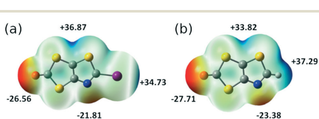
Fig. 3 Molecular electrostatic potential surfaces mapped at 0.001 e ^- au ^{-3} isodensity surface for (a) 2 ; (b) 3 . The common color scale ranges from −28 kcal mol ^{-1} (red) to +40 kcal mol ^{-1} (blue).
