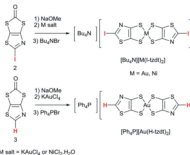
Scheme 3 Synthetic path to the anionic [M(I-tzdt) _2 ] ^- (M = Au, Ni) and [Au(H-tzdt) _2 ] ^- complexes.
