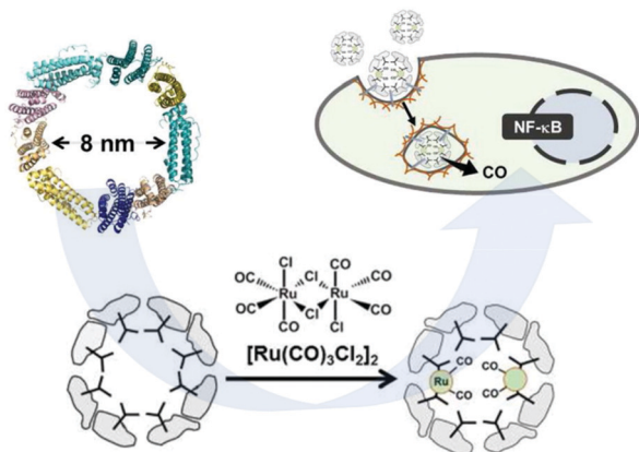
Fig. 9 Schematic representation of the subunit of ferritin with an inner diameter of 8 nm, formation of the \text{Ru(CO)}_2 -protein adduct and cellular uptake of the Ferritin- \text{Ru(CO)}_2 composite and intracellular CO-release. Adapted with permission from ref. 123. Copyright 2014 American Chemical Society.
