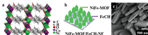
Fig. 4 (a) The overall crystal structure of ultrathin MOF nanosheets of NiCo-MOF (NiCo-UMOFNs), with three coordination structural layers. Reprinted with permission from (ref. 34). Copyright (2016) Springer Nature. (b) A representative diagram of the fabrication of NiFe-MOF/FeCH-NF. (c) SEM image of NiFe-MOF/FeCH-NF. Adapted with permission from ref. 133 with the permission of The Royal Society of Chemistry.
