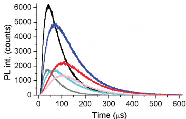
Fig. 5 Time-resolved PL intensities ( \lambda_{em} = 542 \pm 10 nm) of UCNP–DNA nanohybrids without (no FRET) and with (FRET) 3.54 \text{ nmol mg}^{-1} Cy3.5-ssDNA. Black/gray: c-UCNP–DNA without/with Cy3.5-ssDNA ( \lambda_{ex} = 980 nm); blue/cyan: css-UCNP–DNA without/with Cy3.5-ssDNA ( \lambda_{ex} = 980 nm); red/rose: css-UCNP–DNA without/with Cy3.5-ssDNA ( \lambda_{ex} = 808 nm).
