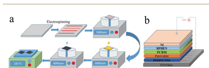
Fig. 19 (a) Schematic illustration of the main fabrication procedure of CuO nanowires. (b) Schematic device structure of the proposed PSC 129 (reprinted with permission from ACS Appl. Mater. Interfaces , 2018, 10 (13), 11289–11296, Copyright 2018 American Chemical Society).
