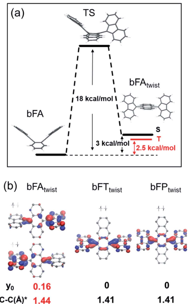
Fig. 5 (a) Energy diagram of bFA with rotation of the fluorene moiety; (b) HOMOs of the fluorene twisted structure of bFA ( \text{bFA}_{\text{twist}} ), bFT ( \text{bFT}_{\text{twist}} ), and bFP ( \text{bFP}_{\text{twist}} ), with the y_0 value and bond length (*) of the C–C bond between fluorene and acenes.
