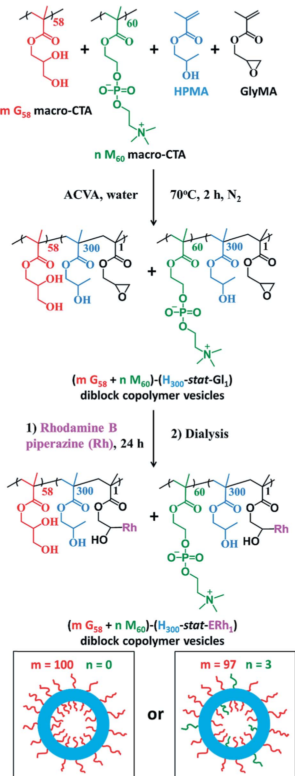
Fig. 1 Synthesis of fluorescently-labelled PGMA_{58} - P(HPMA_{300}\text{-stat-GlyMARh}_1) diblock copolymer vesicles (denoted G_{58}-(H_{300}\text{-stat-ERh}_1) , where m = 100 and n = 0 ) and (97 PGMA_{58} + 3 PMPC_{60}) - P(HPMA_{300}\text{-stat-GlyMARh}_1) diblock copolymer vesicles (denoted (97 G_{58} + 3 M_{60})-(H_{300}\text{-stat-ERh}_1) - D_{52} where m = 97 and n = 3 ) via RAFT aqueous dispersion polymerization. Corresponding schematic cartoons are also shown for each type of precursor vesicle, where PGMA = red, PMPC = green, P(HPMA\text{-stat-ERh}_1) = blue. RAFT end-groups are omitted from chemical structures to aid clarity.
