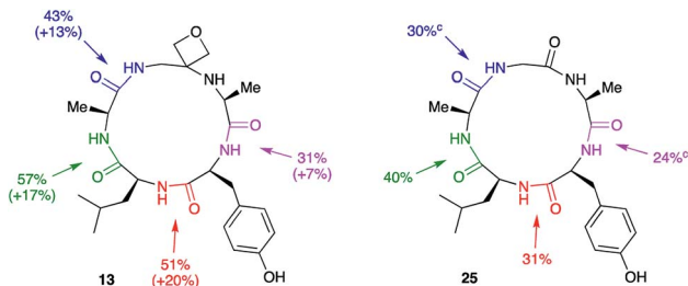
Fig. 5 Macrocyclisation efficiency as a function of location of oxetane relative to forming amide bond. a,b Reaction conditions: DEPBT (2 equiv.), 1 Pr 2 EtN (2 equiv.), DMF (0.001 M), RT, 24 h. a Average of two runs. b Taken from ref. 12.
