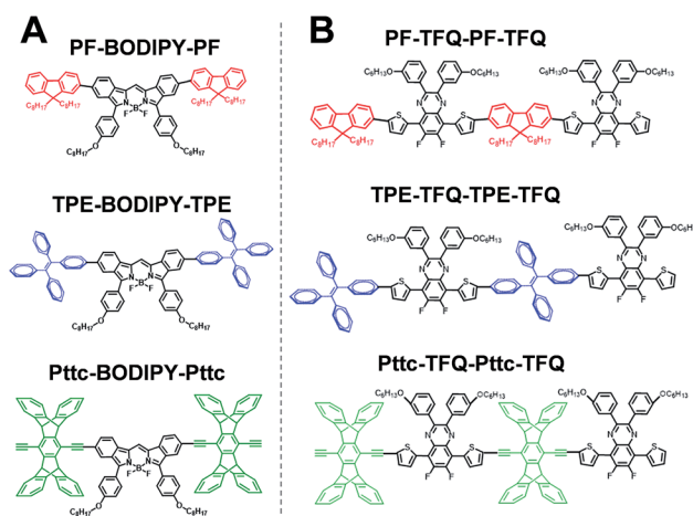
Fig. 3 Chemical structure of (A) donor-acceptor-donor (DAD) oligomers and (B) donor-bridge-donor-bridge (DBDB) oligomers in molecular dynamics simulations: PF-TFQ-BODIPIY (top), TPE-TFQ-BODIPIY (middle), and Pttc-TFQ-BODIPIY (bottom).
