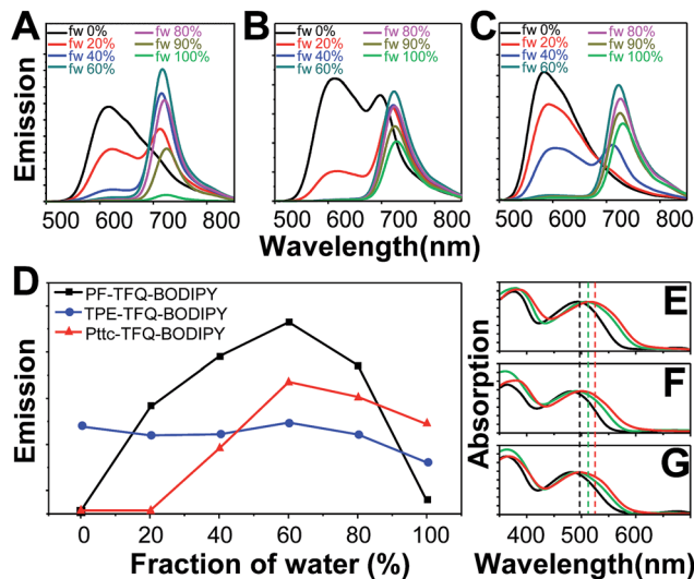
Fig. 2 Emission spectra of the solutions or suspensions containing (A) PF-TFQ-BODIPIY, (B) TPE-TFQ-BODIPIY, and (C) Pttc-TFQ-BODIPIY polymers in THF/water mixtures with different volumetric fractions of water (fw, vol%). (D) Response of BODIPIY fluorescence intensities ( \sim 724 nm) for the three polymers in mixed solvents of THF/water (water fraction, v/v%). Normalized absorption spectra of (E) PF-TFQ-BODIPIY, (F) TPE-TFQ-BODIPIY, and (G) Pttc-TFQ-BODIPIY in pure \text{CH}_2\text{Cl}_2 (black lines), Pdot aqueous form (green lines), and film form (red lines).
