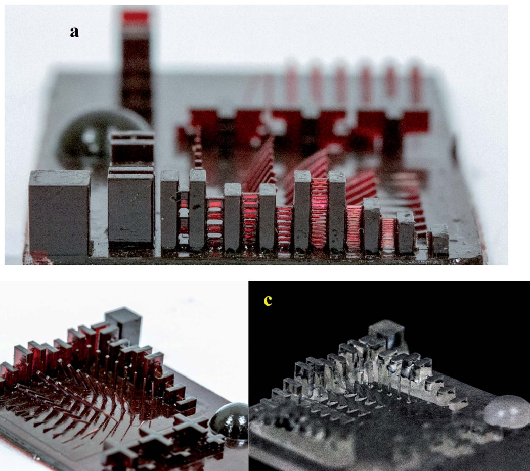
Fig. 4 Photographs of the printed benchmark design for (a) 3KSRD sample (Z-resolution), (b) 3KSRD sample and (c) 1KTPO sample.
