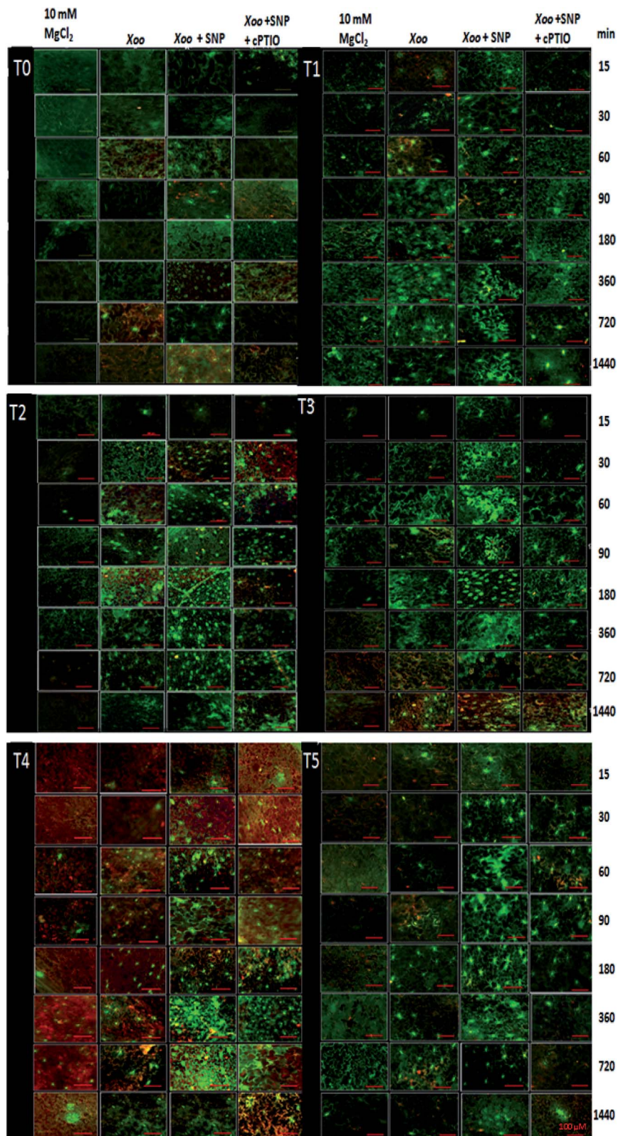
Fig. 8 Detection of NO accumulation using diaminofluorescein-FM fluorescence in tobacco leaves after Xoo infiltration. Xoo-induced DAF-FM T fluorescence under different treatments: dist. H 2 O (T0), T42 treated (T1), nitrate (T2), nitrate + T42 strain (T3), ammonium (T4) and ammonium + T42 strain (T5) grown tobacco leaves. After preloading cells with DAF-FM (as described in the Experimental setup section), Xoo suspension culture singly, Xoo + 100 μM SNP, and Xoo + 100 μM SNP + 200 μM cPTIO were infiltrated. Cell suspensions for Xoo were prepared in 10 mM MgCl 2 and infiltration of MgCl 2 served as a control. At the indicated times, 0.75 cm 2 discs were removed from the leaves for fluorescence observation. Note that the reaction product of DAF and NO, DAF-FM T, is stable for a long time. Therefore, a continuous increase in fluorescence indicates a constant rate of NO formation. Bars represent = 100 μm.
