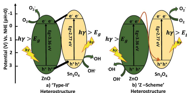
Fig. 11 Schematic diagram of electron transfer in the \text{ZnO}@ \text{Sn}_3\text{O}_4 .
