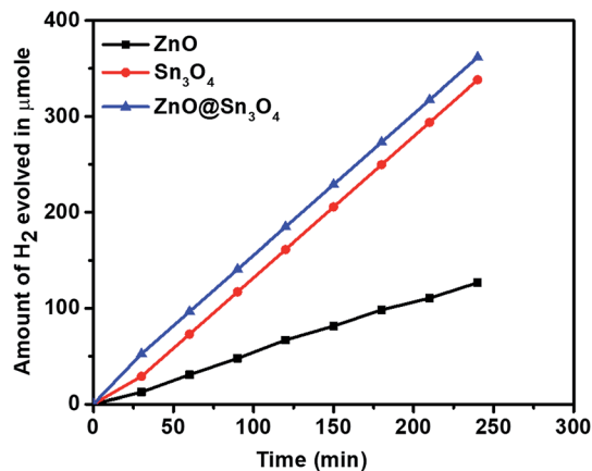
Fig. 10 Hydrogen production as a function of irradiation time in the presence of ZnO, \text{Sn}_3\text{O}_4 and \text{ZnO}@ \text{Sn}_3\text{O}_4 .
