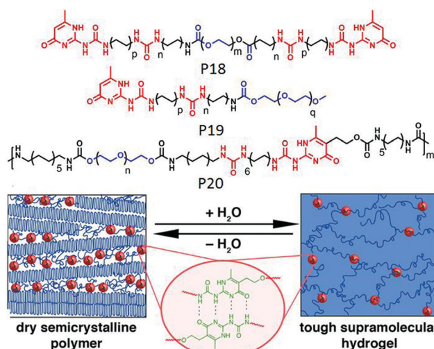
Fig. 22 Structure of P18 , P19 and P20 and schematic representation of cross-linked hydrogel and phase separated domain in a dry polymer. Adapted with permission from ref. 67. Copyright 2014, American Chemical Society.
