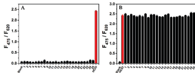
Fig. 3 (A) Fluorescence intensity ratio ( F_{475}/F_{620} ) for AIED-Lyso ( 2.67 \mu\text{g mL}^{-1} ) in the presence of 20 \mu\text{M} HClO or one biologically relevant molecule; (B) fluorescence intensity ratio ( F_{475}/F_{620} ) for AIED-Lyso ( 2.67 \mu\text{g mL}^{-1} ) in the presence of 20 \mu\text{M} of HClO and one biologically relevant molecule; note: (1–18: 200 \mu\text{M} , 19–20: 5.0 mM, 21–25: 200 \mu\text{M} ) 1, \text{Na}^+ ; 2, \text{K}^+ ; 3, \text{Ca}^{2+} ; 4, \text{Zn}^{2+} ; 5, \text{Co}^{2+} ; 6, \text{Cu}^{2+} ; 7, \text{Mg}^{2+} ; 8, \text{Fe}^{3+} ; 9, \text{Fe}^{2+} ; 10, \text{Ni}^{2+} ; 11, \text{Cl}^- ; 12, \text{SO}_4^{2-} ; 13, \text{NO}_3^- ; 14, \text{H}_2\text{PO}_4^- ; 15, \text{HPO}_4^{2-} ; 16, \text{PO}_4^{3-} ; 17, \text{SO}_3^{2-} ; 18, \text{NO}_2^- ; 19, Cys; 20, GSH; 21, \text{H}_2\text{O}_2 ; 22, NO; 23, ^1\text{O}_2 ; 24, HO; 25, t\text{-BuO} . \lambda_{\text{ex}} = 399 nm.
