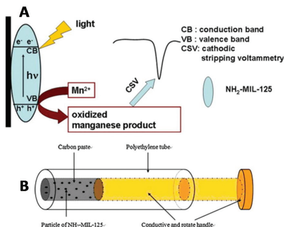
Fig. 6 (A) The photooxidation procedure of Mn^{2+} at the NH_2 -MIL-125-Ti/CPE and its determination by CSV. (B) Schematic illustration of the structure of the NH_2 -MIL-125(Ti) modified carbon paste electrode. Reprinted from ref. 72d with permission from Elsevier.
