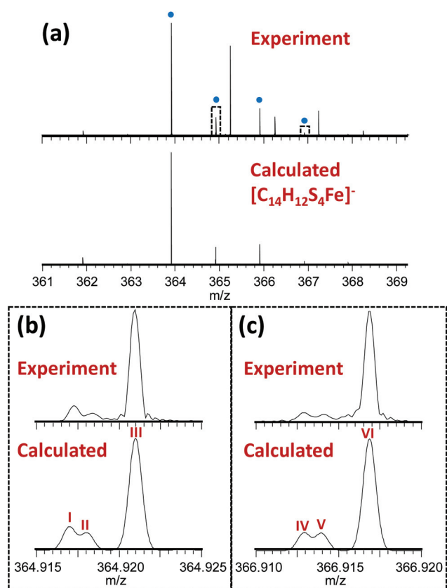
Fig. 1 (a) Observed mass spectrum of [\text{Fe(4-methyl-1,2-benzenedithiolate)}_2]^- (peaks labelled with blue dots) and comparison with the calculated isotope distribution. Unlabelled peaks are due to a contaminant present in the solvent (MeOH), (see Fig. S1, Table S2, ESI†). Panels (b) and (c) show zoomed-in views (10 mDa wide) of the peaks near 364.92 and 366.92 m/z (indicated by dotted rectangles in Panel A) illustrating a good match between the theoretical and observed isotopic fine structure indicating high confidence in the assigned elemental compositions. These fine structure peaks were assigned as follows: I – [\text{C}_{14}^{12}\text{C}_{14}^{13}\text{H}_{12}^{1}\text{H}_{12}^{2}\text{S}_3^{32}\text{S}_3^{33}\text{S}_4^{56}\text{Fe}]^- ; II – [\text{C}_{14}^{12}\text{C}_{14}^{13}\text{H}_{12}^{1}\text{H}_{12}^{2}\text{S}_4^{32}\text{S}_4^{33}\text{S}_4^{57}\text{Fe}]^- ; III – [\text{C}_{13}^{12}\text{C}_{13}^{13}\text{C}_{14}^{1}\text{H}_{12}^{1}\text{H}_{12}^{2}\text{S}_4^{32}\text{S}_4^{33}\text{S}_4^{56}\text{Fe}]^- ; IV – [\text{C}_{14}^{12}\text{C}_{14}^{13}\text{H}_{12}^{1}\text{H}_{12}^{2}\text{S}_2^{32}\text{S}_2^{33}\text{S}_4^{34}\text{S}_4^{56}\text{Fe}]^- ; V – [\text{C}_{14}^{12}\text{C}_{14}^{13}\text{H}_{12}^{1}\text{H}_{12}^{2}\text{S}_3^{32}\text{S}_3^{33}\text{S}_4^{34}\text{S}_4^{57}\text{Fe}]^- ; VI – [\text{C}_{13}^{12}\text{C}_{13}^{13}\text{C}_{14}^{1}\text{H}_{12}^{1}\text{H}_{12}^{2}\text{S}_3^{32}\text{S}_3^{33}\text{S}_4^{34}\text{S}_4^{56}\text{Fe}]^- . Note that the spectra in panels (b) and (c) are effectively expanded 400-fold compared to panel (a), explaining why the additional fine structure peaks are not visible in the top spectrum.
