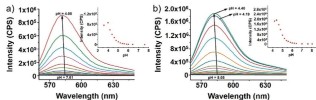
Fig. 9 (a) Fluorescence spectral changes of probe 6 (5 \mu M) in Britton–Robinson buffer (B–R buffer) solution at different pH values ( \lambda_{\text{ex}} = 540 nm), and the maximum emission intensity was measured at 583 nm. Inset: Plot of the emission fluorescence intensity at 583 nm; pH 3.60, 4.00, 4.19, 4.40, 4.62, 4.80, 5.01, 5.21, 5.41, 5.59, 5.82, 6.00, 6.21, 6.42, 7.01, and 7.61. (b) Fluorescence spectral changes of probe 7 (5 \mu M) in B–R buffer solution at different pH values ( \lambda_{\text{ex}} = 540 nm), and the maximum emission fluorescence intensity was measured at 583 nm. Inset: Plot of the emission fluorescence intensity at 583 nm; pH 3.60, 4.00, 4.19, 4.40, 4.62, 4.80, 5.01, 5.21, 5.41, 5.59, 5.82, 6.00, 6.21, 6.42, 7.01, 7.61, and 8.05. Copyright 2014 Royal Society of Chemistry.
