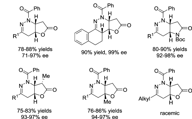
Scheme 10 Cu(II)/tBu-Box catalyzed formal [4+2] annulation of azoalkene with 2-silyloxyfuran.
