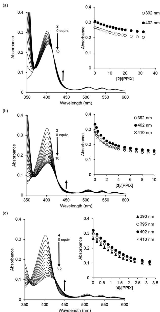
Fig. 3 UV-Vis titrations of PPIX (2.4 \mu\text{M} ) with (a) 2 , (b) 3 , and (c) 4 in \text{DMSO}/33 \text{ mM} HEPES buffer (pH 7.4) = 2 : 3 (v/v) at 25 °C. Insets: changes in the absorbance of PPIX upon the addition of compounds 2–4.
