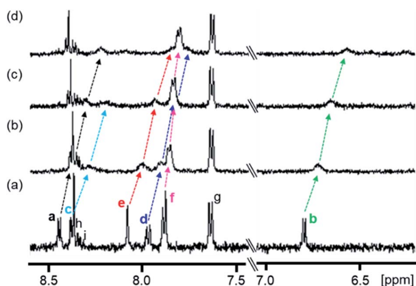
Fig. 2 Partial ^1\text{H} NMR spectra (500 MHz) of 1 in the absence and presence of PPIX in \text{DMSO}-d_6/33 \text{ mM} HEPES buffer (pD 7.4) = 2 : 1 (v/v) at 23 °C. (a) 1 (0.10 mM), (b) 1 (0.10 mM) + PPIX (0.020 mM), (c) 1 (0.10 mM) + PPIX (0.050 mM) and (d) 1 (0.10 mM) + PPIX (0.10 mM). 1% tetramethylsilane in \text{CCl}_4 was used as the external reference. Peak assignments of aromatic protons \text{H}^{\text{a}}-\text{H}^{\text{i}} on 1 are listed in Scheme 3.
